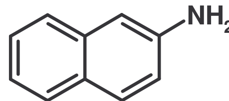
\beta -naftylamin
